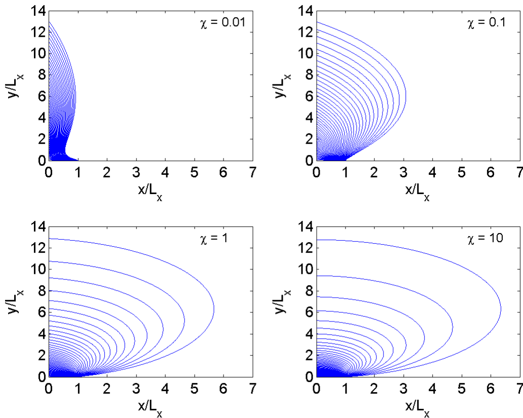
Fig. 4.2. Effect of the streambed conductance coefficient \chi on the streamlines for \kappa_y = 1 . The well is at (x/L_x, y/L_x) = (1, 0) , the river is at x/L_x = 0 , and the fraction of flow between adjacent streamlines is constant.
